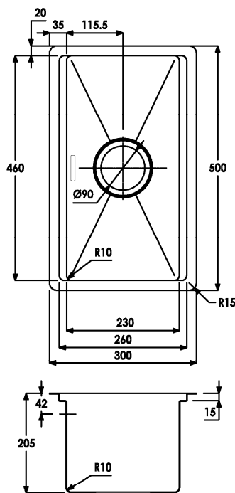
UNDERMOUNT CUT OUT
